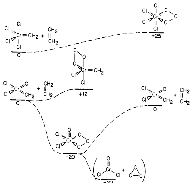
Figure 1. Energetics ( \Delta G_{300} in kcal/mol) for the reaction of C_2H_4 with the carbene and oxo-alkylidene of Cr.
