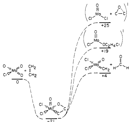
Figure 11. Energetics ( \Delta G_{300} in kcal/mol) for the reaction of C_2H_4 with molybdenyl chloride.
