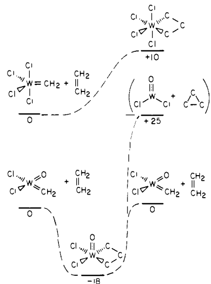
Figure 3. Energetics ( \Delta G_{300} in kcal/mol) for the reaction of C_2H_4 with the carbene and oxo-alkylidene of W.
