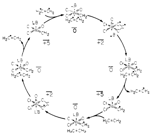
Figure 8. The full catalytic cycle for metathesis by W oxo-alkylidene with Lewis base present (energies are \Delta G_{300} in kcal/mol).
