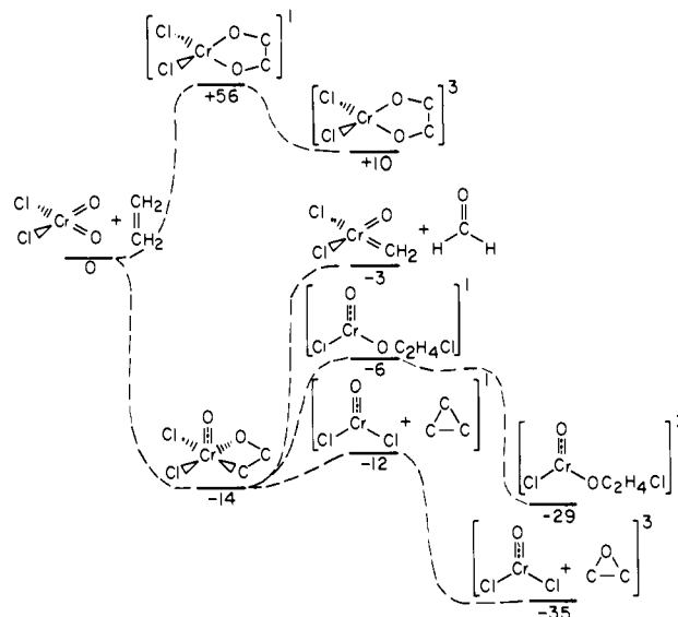
Figure 10. Energetics ( \Delta G_{300} in kcal/mol) for the reaction of C_2H_4 with chromyl chloride.
