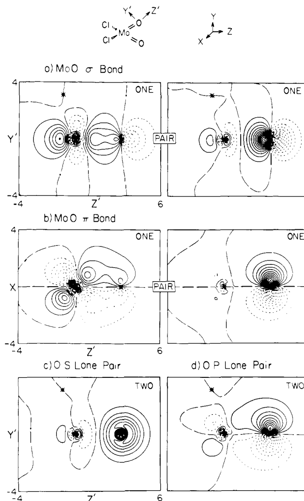
Figure 4. The GVB orbitals involved in the bond to one oxo group of (\text{Cl})_2\text{Mo}(\text{=O})_2 . The long dashes indicate zero amplitude and dotted lines indicate negative amplitude. The spacing between contours is 0.0625 au.
