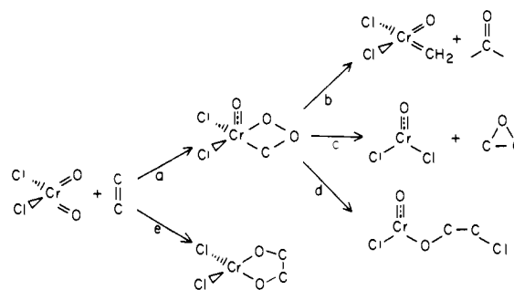
Figure 10. Energetics ( \Delta G_{300} in kcal/mol) for the reaction of C_2H_4 with chromyl chloride.
