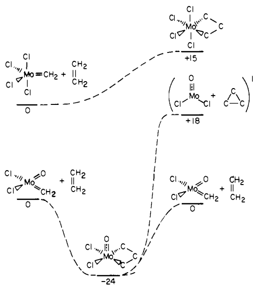
Figure 2. Energetics ( \Delta G_{300} in kcal/mol) for the reaction of C_2H_4 with the carbene and oxo-alkylidene of Mo.
