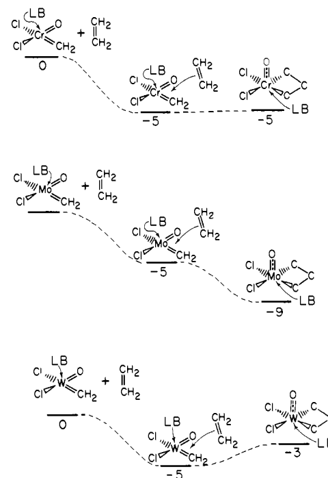
Figure 6. Effect of a Lewis base (LB) and \pi complexation of the olefin upon the energetics ( \Delta G_{300} in kcal/mol) for the reaction of C 2 H 4 with oxo-alkylidenes.
