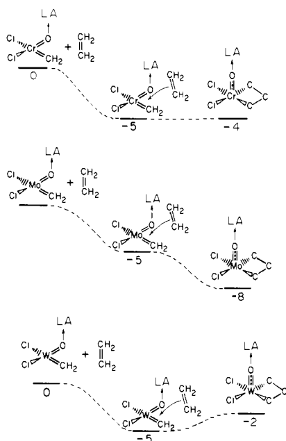
Figure 7. Effect of a Lewis acid (LA) and \pi complexation of the olefin upon the energetics ( \Delta G_{300} in kcal/mol) for the reaction of C_2H_4 with oxo-alkylidenes.
