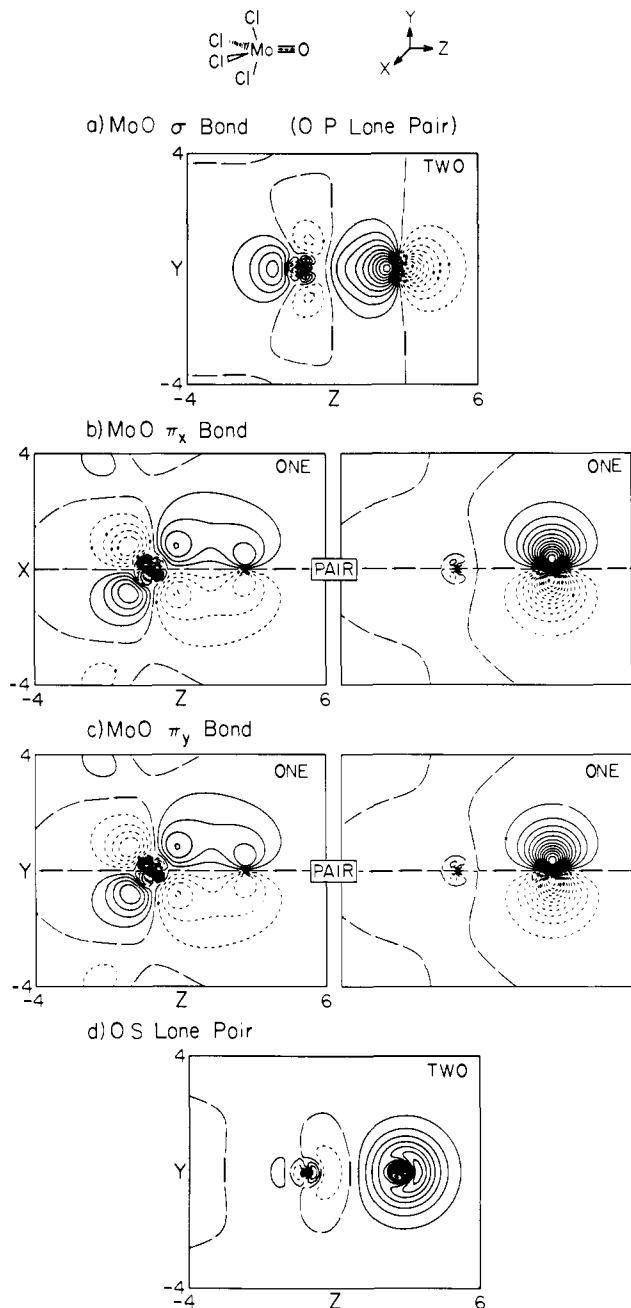
Figure 5. The GVB orbitals involved in the oxo bond of Cl 4 Mo=O.
