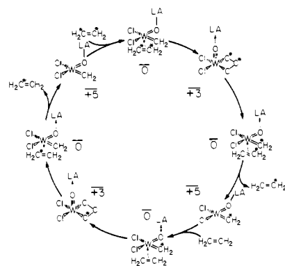
Figure 9. The full catalytic cycle for metathesis by W oxo-alkylidene with Lewis acid present (energies are \Delta G_{300} in kcal/mol).
